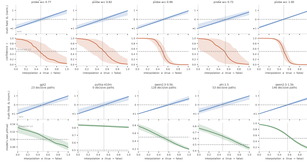
Figure 2: Upper pair of rows, the truth probe (normalized, median and interquartile band) and the independently trained confidence along true-to-negation paths, the dotted line marking the mean probe zero crossing where confidence passes near one half. Lower pair, the same with the model’s own probability of answering true from patched final-block states, decisive paths where any exist. The Qwens sweep through one half at the boundary, Pythia-410M answers true everywhere so the premise fails, and GPT-2 and Phi-1.5 sit between.
