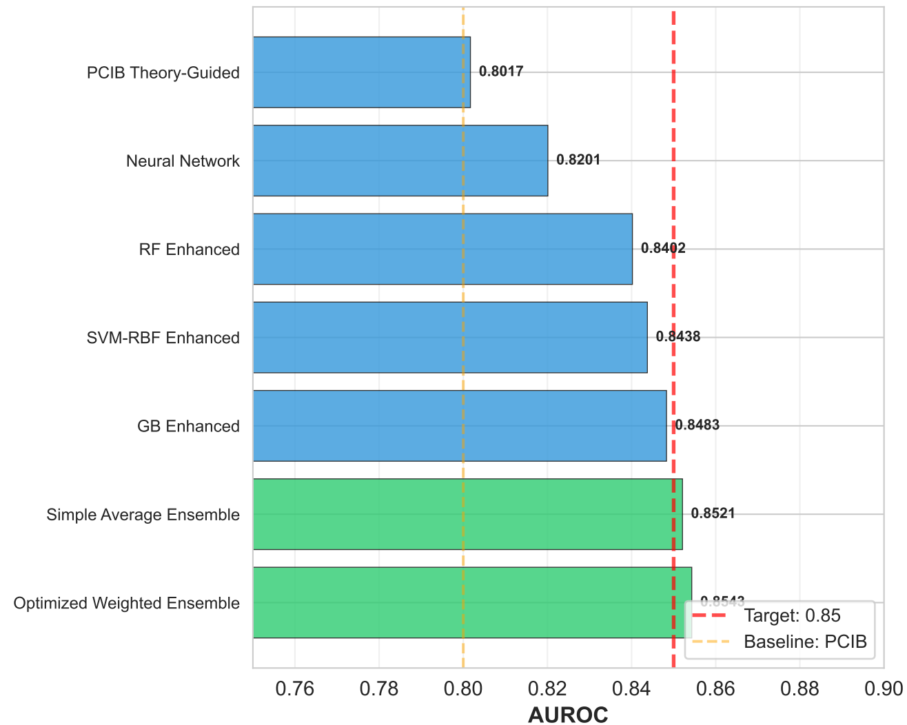
AUROC Performance
