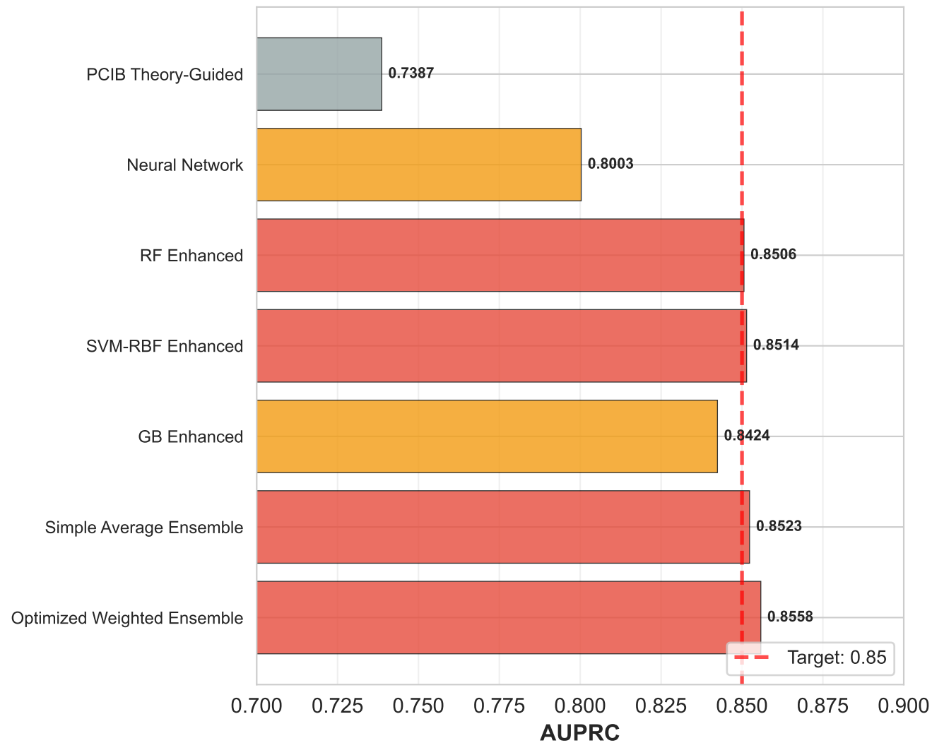
AUPRC Performance
