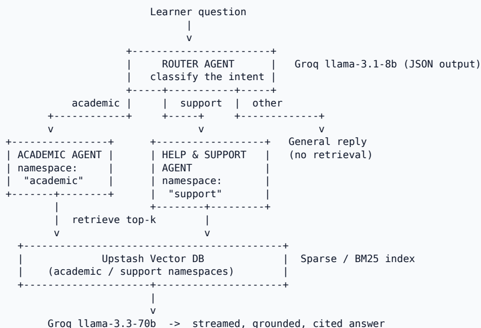
Fig 1. Orchestrator routes each query to one specialist, which retrieves from its own namespace.
