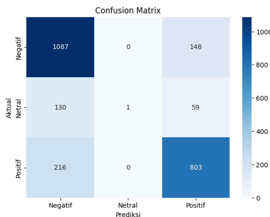
Confusion Matrix
