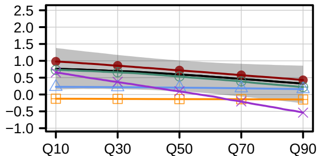
EPL ( \varsigma )
