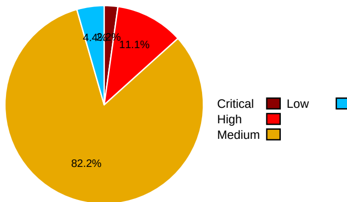
Vulnerabilities Distribution (%)
