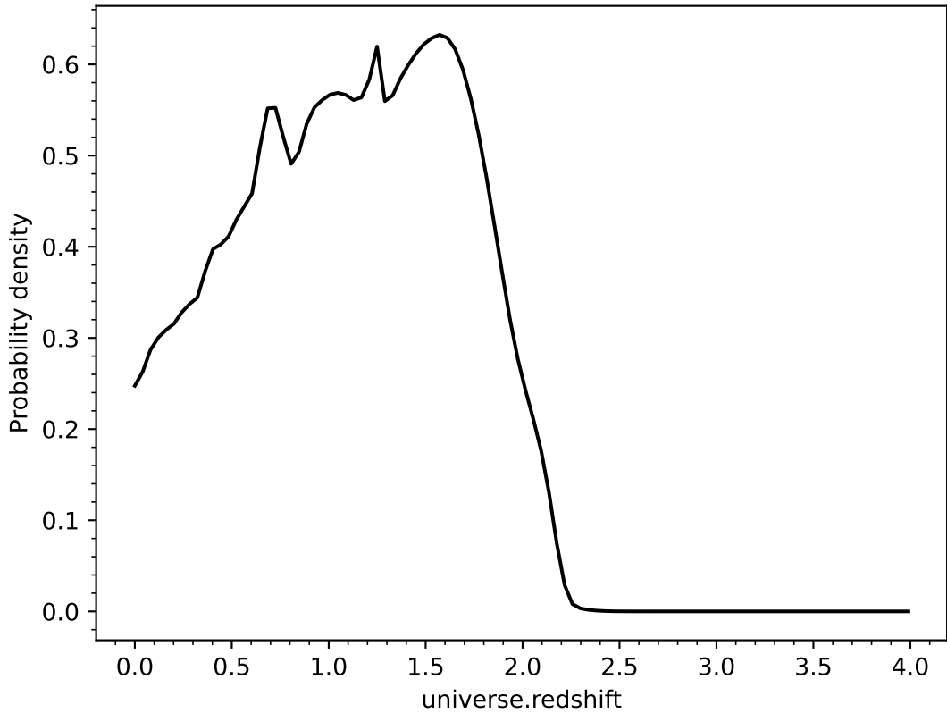
Probability distribution function of universe.redshift for 0
