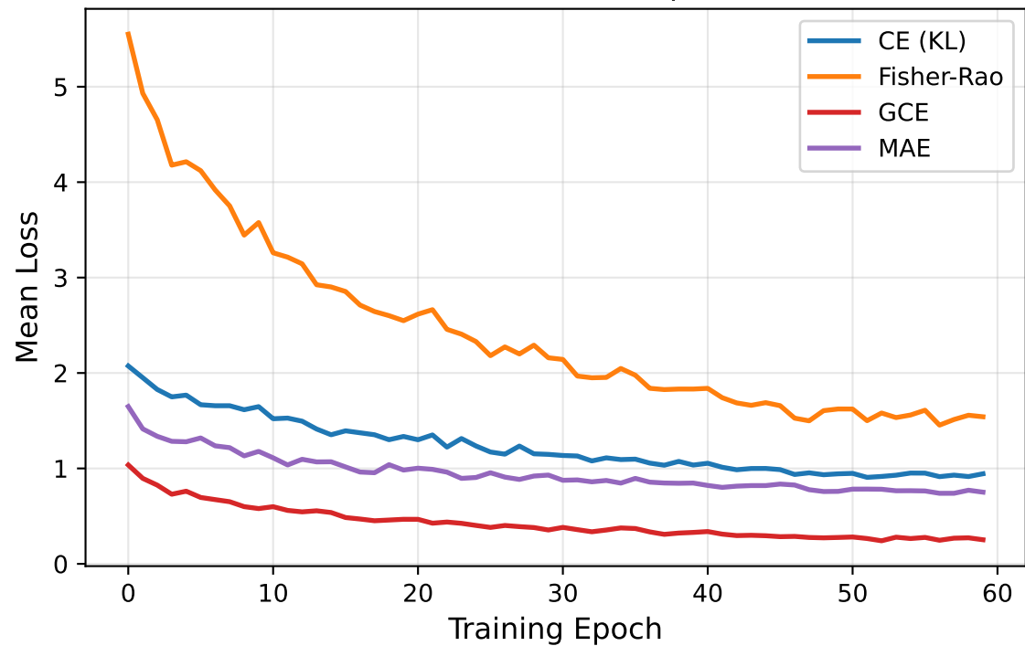
Loss — Clean Samples
