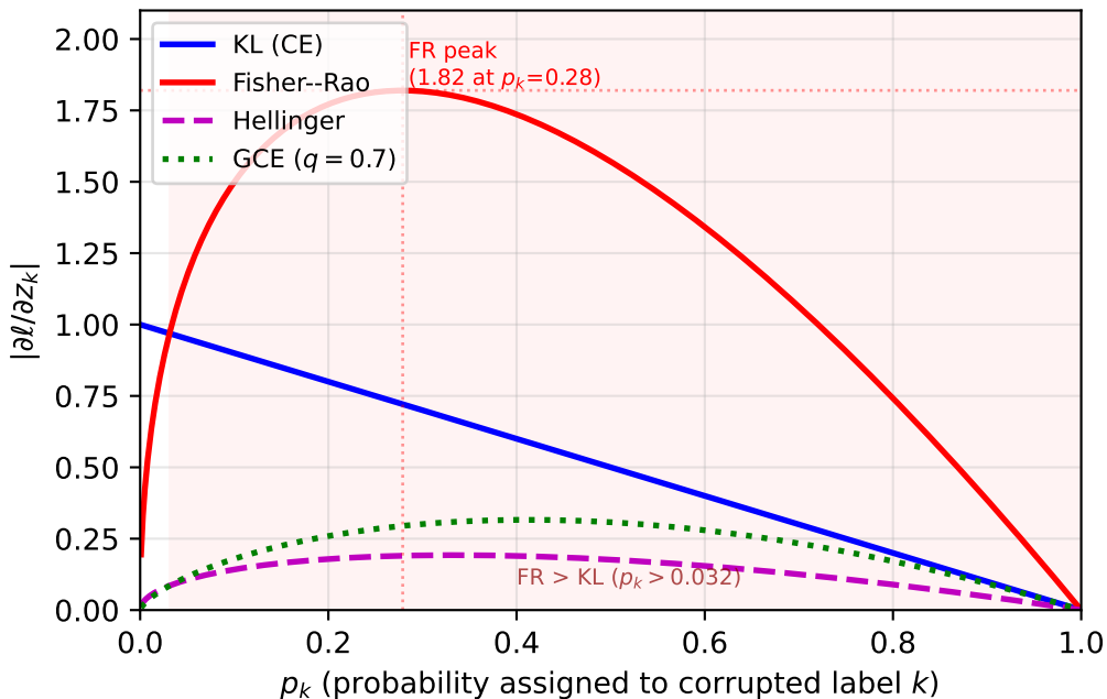
Gradient magnitude vs. predicted probability
