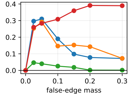
bad-edge preservation
