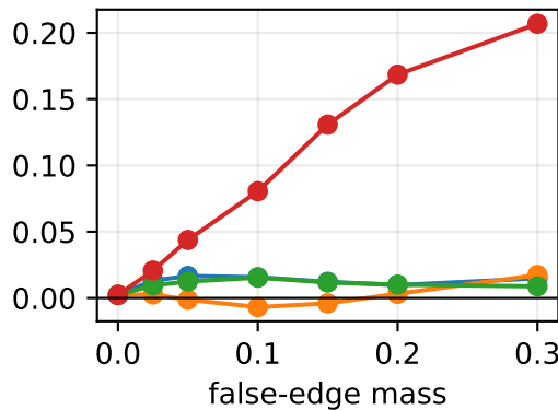
trustworthiness
