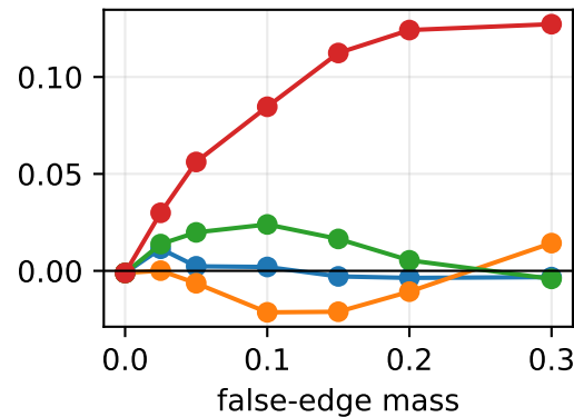
clean-neighbor recall
