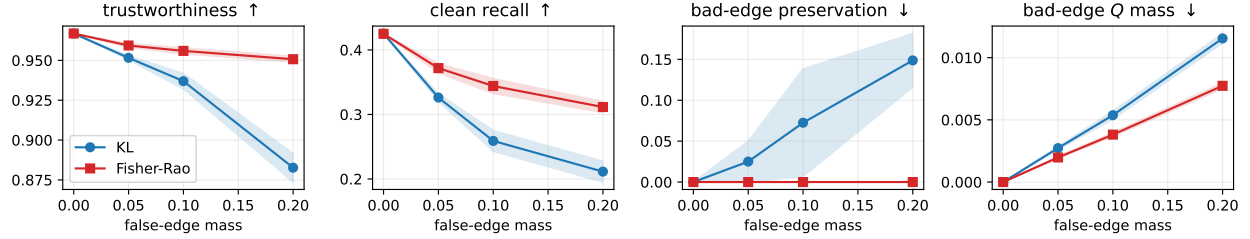
Figure 7: Noisy-affinity stress test under injected false high-probability edges. Unlike feature-noise corruption, this directly contaminates the target pair distribution. KL increasingly preserves the injected bad edges as false-edge mass grows, while Fisher–Rao maintains higher clean-neighborhood metrics and assigns less embedding probability to the corrupted pairs.
