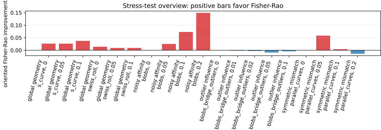
Figure 9: Stress-test overview. Each bar is oriented so positive means Fisher–Rao improves the most diagnostic metric for that stress family. The clearest signal is the noisy-affinity false-edge benchmark; other stress families are weaker or mixed.
