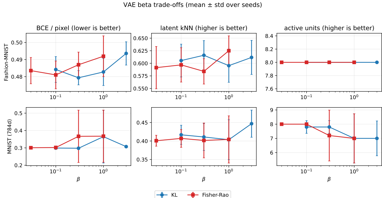
Figure 10: VAE beta trade-offs across reconstruction, latent kNN accuracy, and active units. Curves show mean \pm 1 standard deviation across five seeds for each dataset and regularizer.
