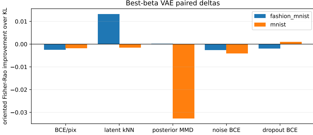
Figure 11: Best-beta paired VAE deltas. Values are oriented so positive means Fisher–Rao is better: lower BCE/MMD is multiplied by -1 , while higher latent accuracy is left positive.
