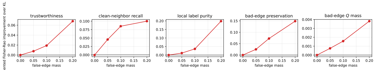
Structured false-affinity robustness: Fisher-Rao resists corrupted edges
