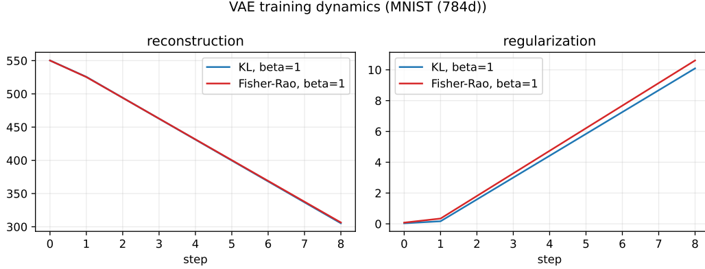
Figure 12: VAE training dynamics on MNIST for the representative \beta = 1 setting. Raw KL and Fisher–Rao regularization values are not directly comparable in scale, but both optimize smoothly under Adam after gradient clipping.
