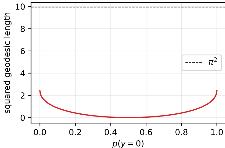
d_{\text{FR}}(p, q)^2 (bounded by \pi^2 )
