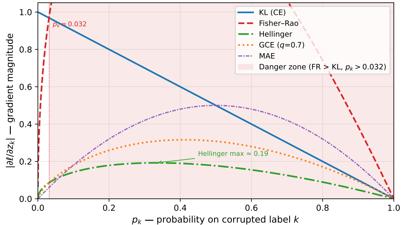
Gradient magnitude on corrupted label vs. confidence p_k (shaded: danger zone where FR amplifies corrupted gradients above KL)
