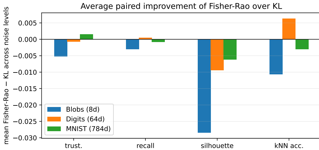
Figure 14: Average paired improvement of Fisher-Rao over KL for each metric, averaged across noise levels, broken down by dataset. Bars below zero mean KL is better on average.
