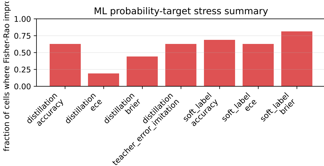
Figure 12: Fraction of nonzero corruption cells where Fisher-Rao improves over KL for the supervised probability-target stress tests.
