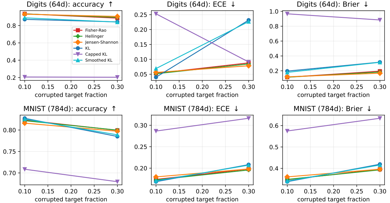
Figure 10: Noisy soft-label classification under adversarial overconfident target corruption. Fisher-Rao is most useful when KL overfits wrong high-confidence probability labels; bounded alternatives such as Hellinger and Jensen-Shannon provide important baselines.
