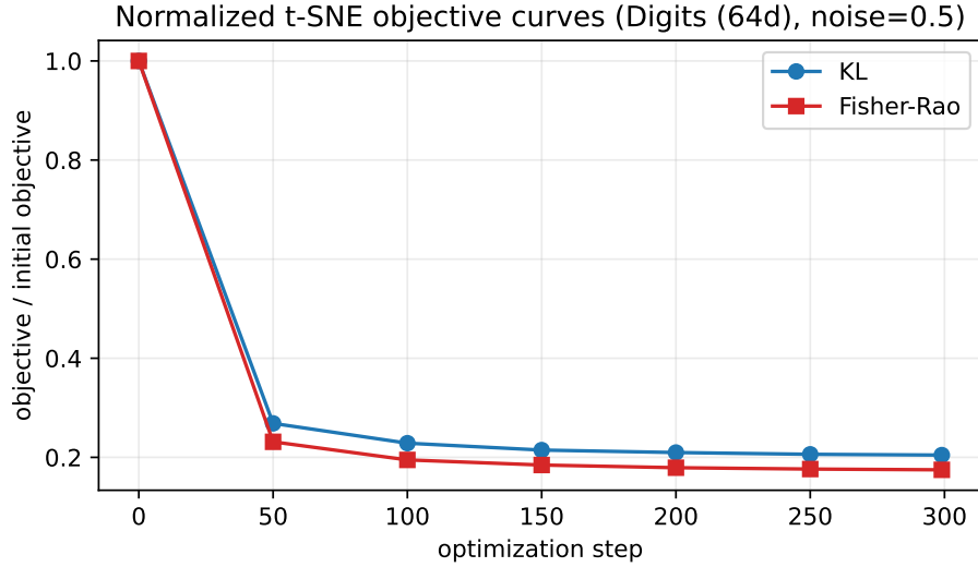
Figure 16: Normalized t-SNE objective curves on digits at noise \alpha = 0.5 . Both objectives are well-behaved under Adam; the relative decrease rates differ because the underlying loss landscapes have different scales.
