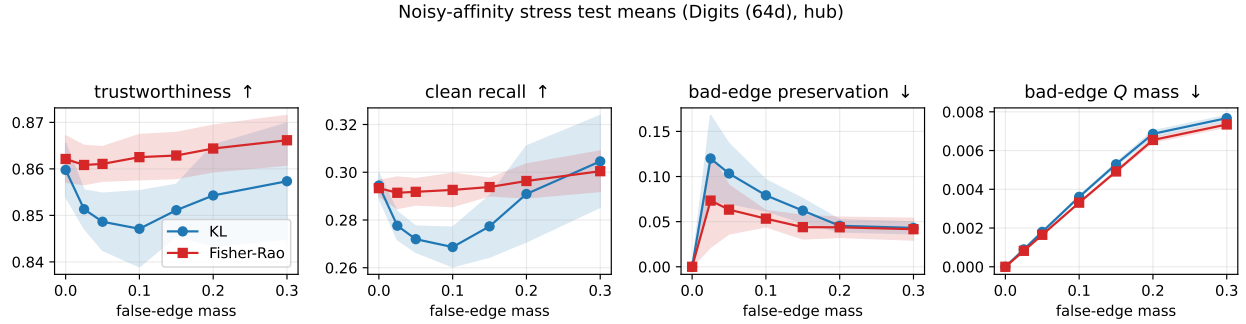
Figure 4: Noisy-affinity stress test under injected false high-probability edges. Unlike feature-noise corruption, this directly contaminates the target pair distribution. KL increasingly preserves the injected bad edges as false-edge mass grows, while Fisher–Rao maintains higher clean-neighborhood metrics and assigns less embedding probability to the corrupted pairs.
