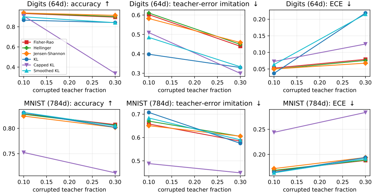
Figure 11: Corrupted teacher-student distillation. Fisher-Rao can reduce imitation of teacher mistakes, but the result is less uniform than the soft-label benchmark.
