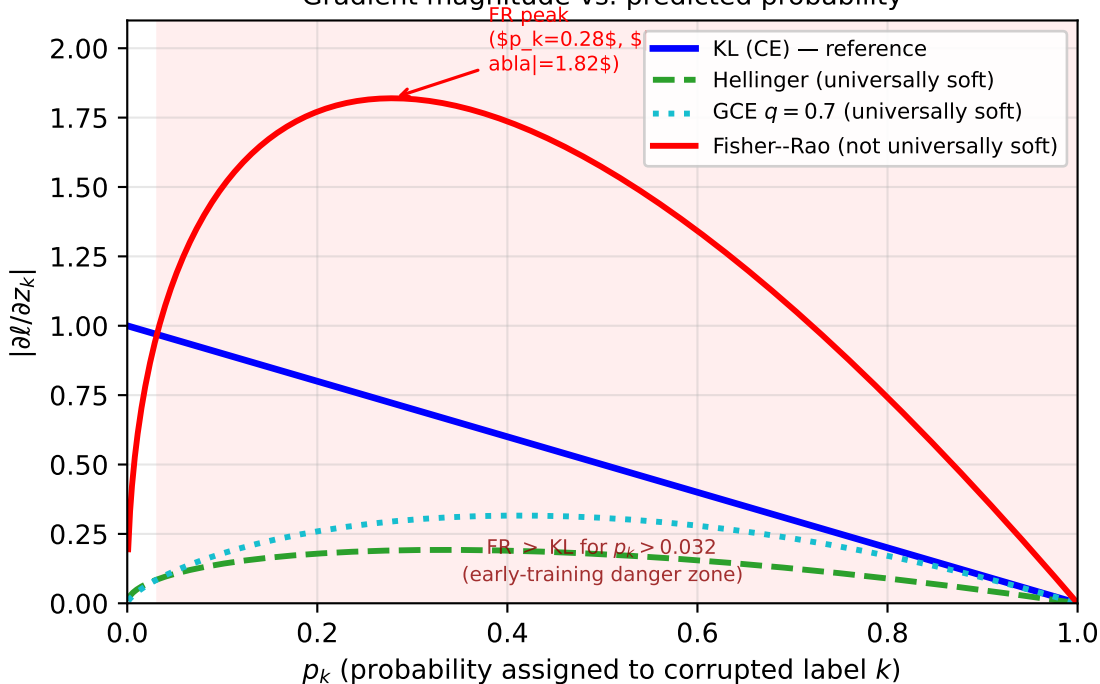
Gradient magnitude vs. predicted probability
