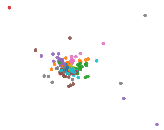
Fisher-Rao, noise=0.0
