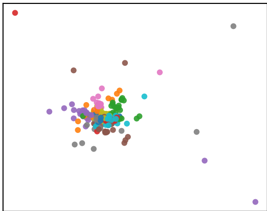
Fisher-Rao, noise=0.0
