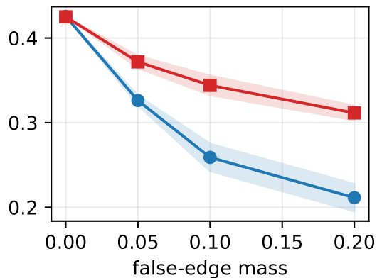
clean recall \uparrow
