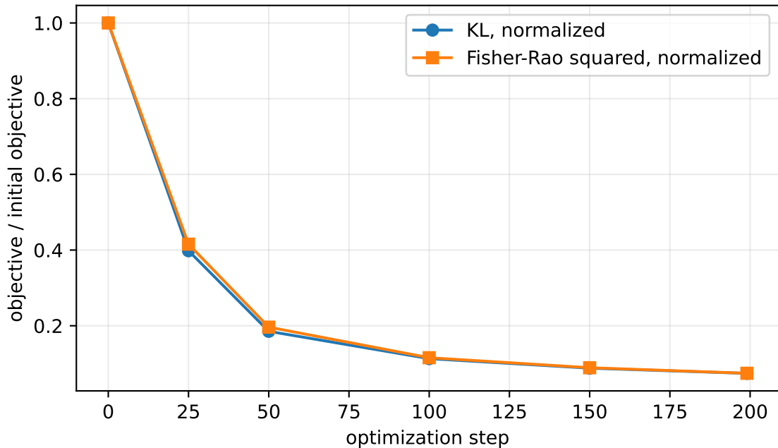
t-SNE objective decrease
