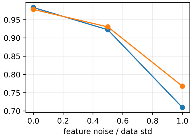
trustworthiness
