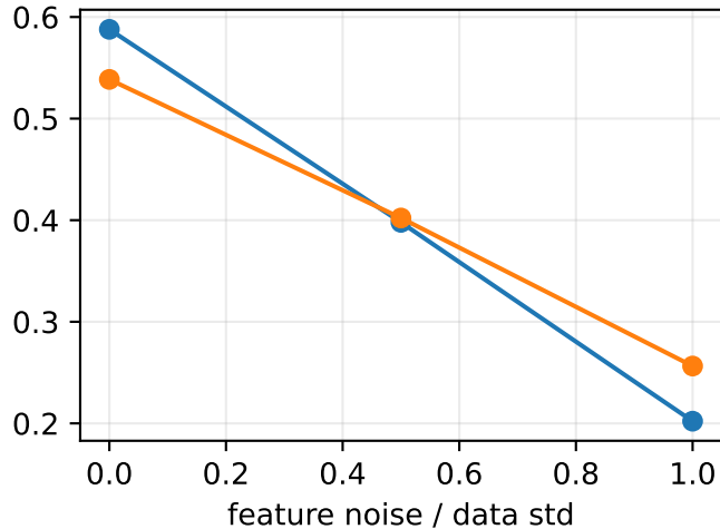
neighborhood recall
