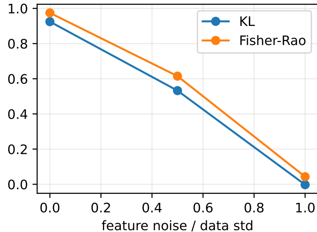
silhouette
