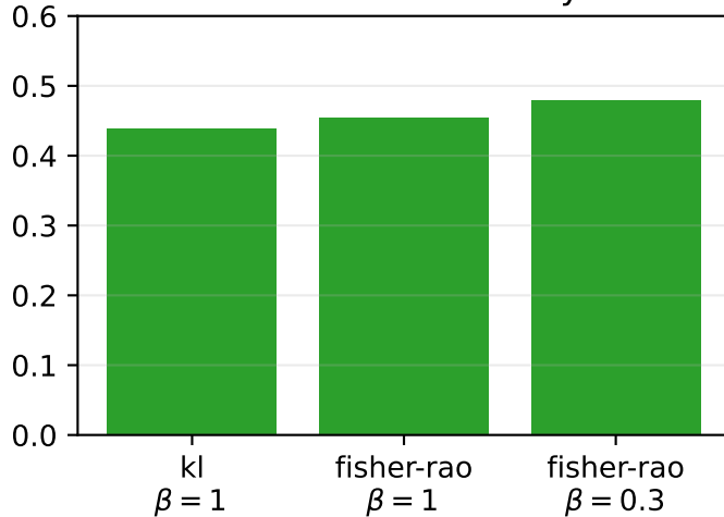
latent kNN accuracy
