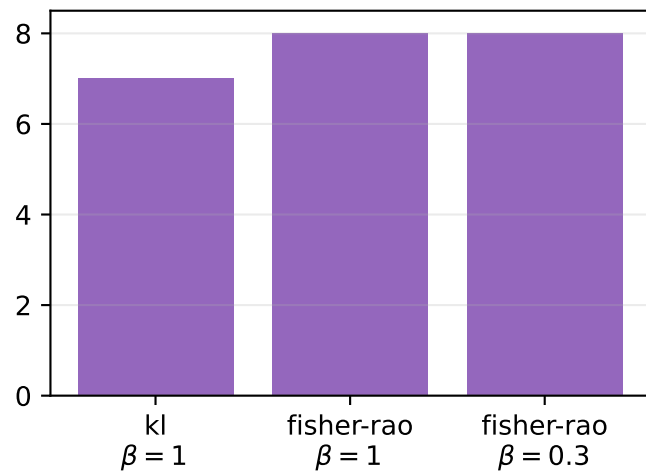
active latent units
