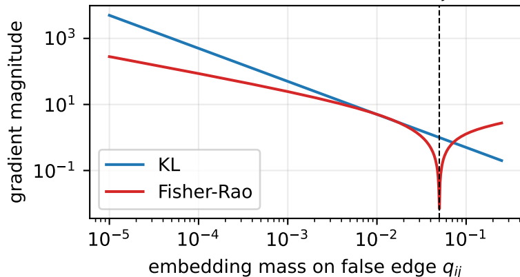
KL pressure grows as 1/q_{ij}
