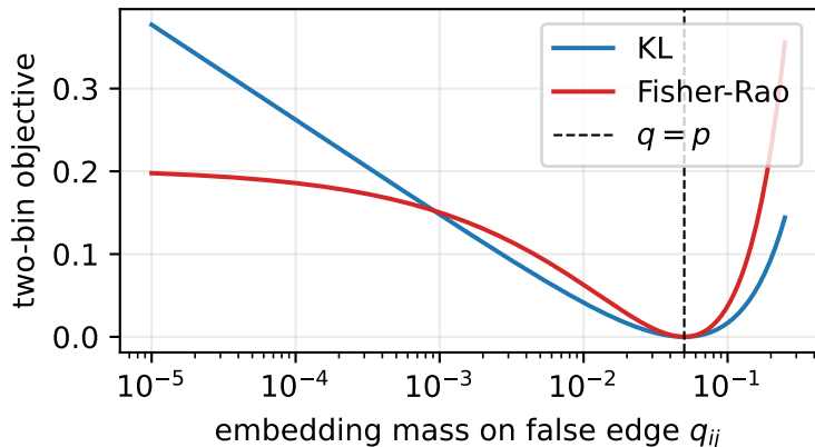
False-edge objective shape
