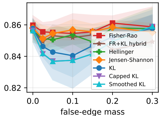
trustworthiness \uparrow
