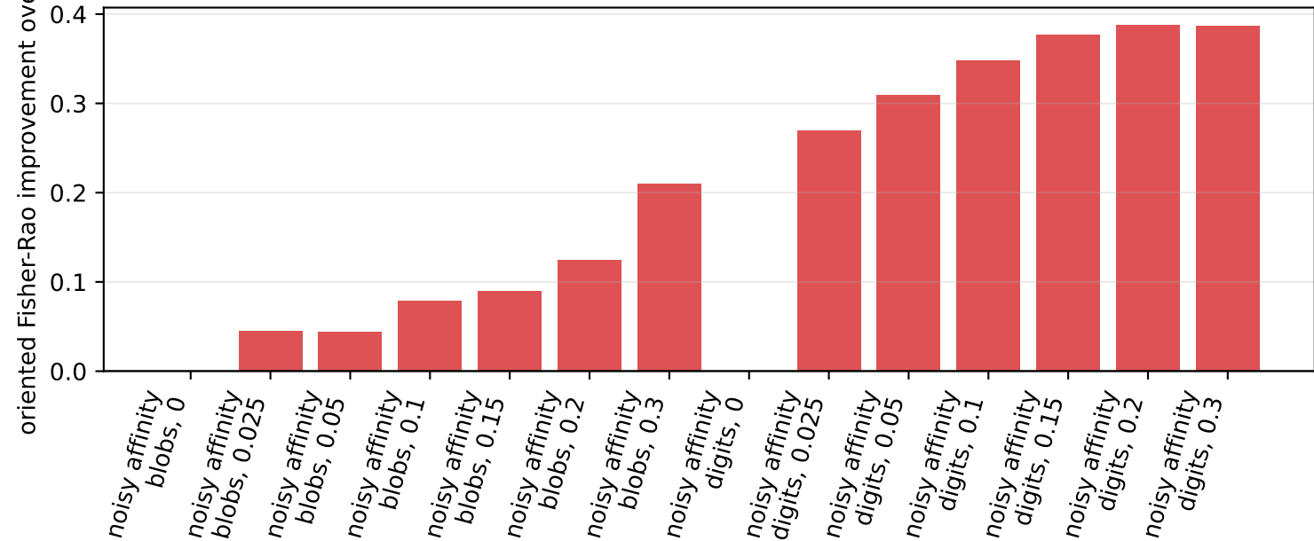
Stress-test overview: positive bars favor Fisher-Rao
