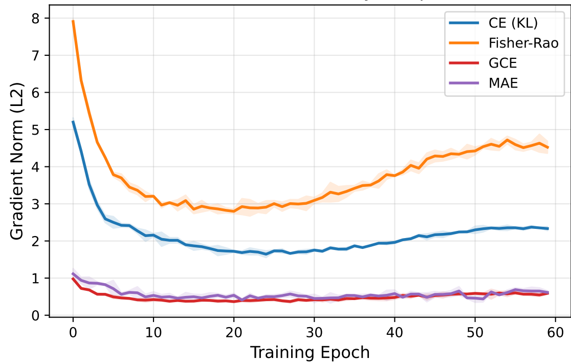
Gradient Norm — Noisy Samples
