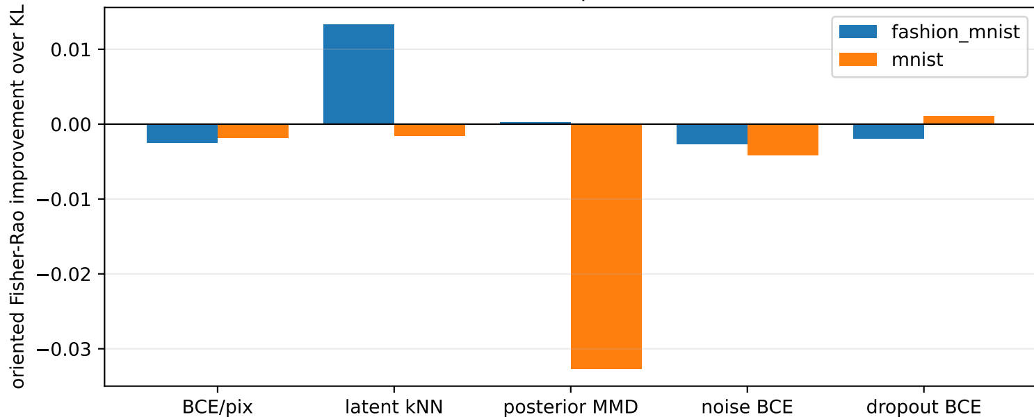
Best-beta VAE paired deltas
