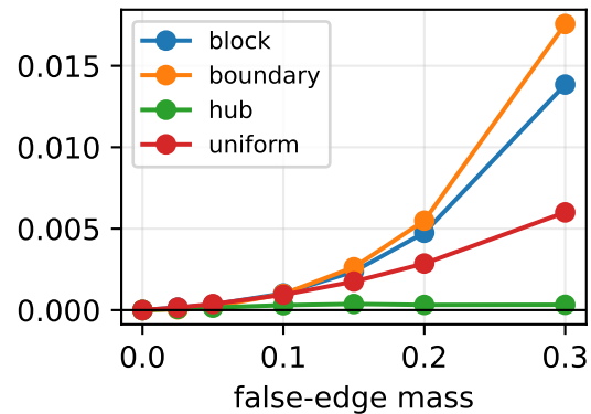
bad-edge Q mass
