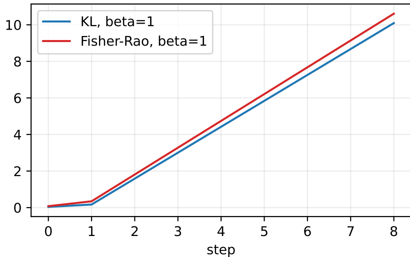
regularization
