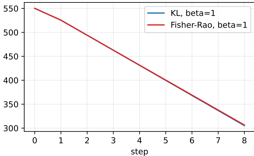
reconstruction
