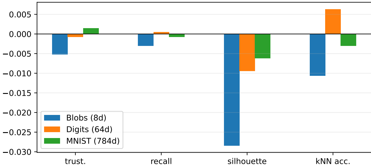
Average paired improvement of Fisher-Rao over KL
