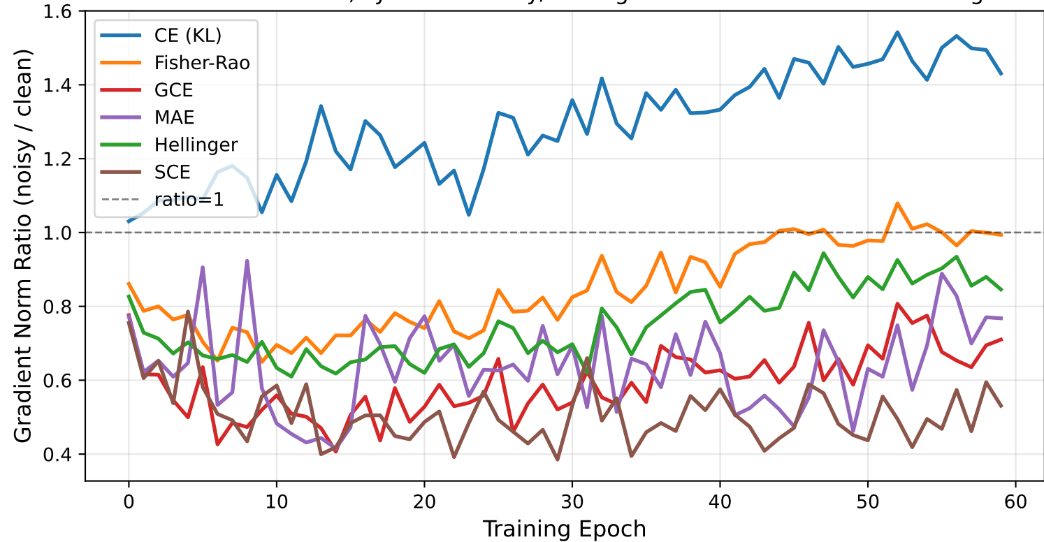
CIFAR-10 ConvNet, sym 40%: noisy/clean gradient norm ratio over training
