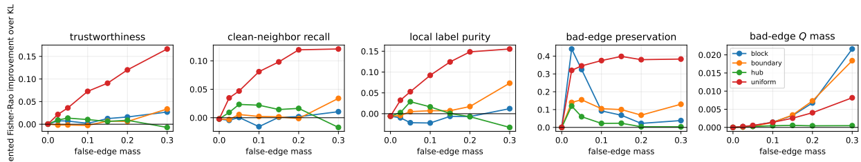
Structured false-affinity robustness on Digits (64d)
