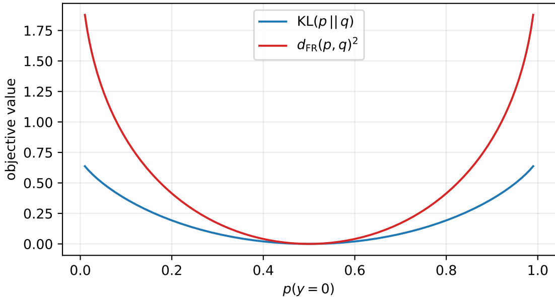
Categorical two-class objective shape
