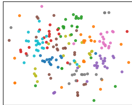
Fisher-Rao, noise=1.0
