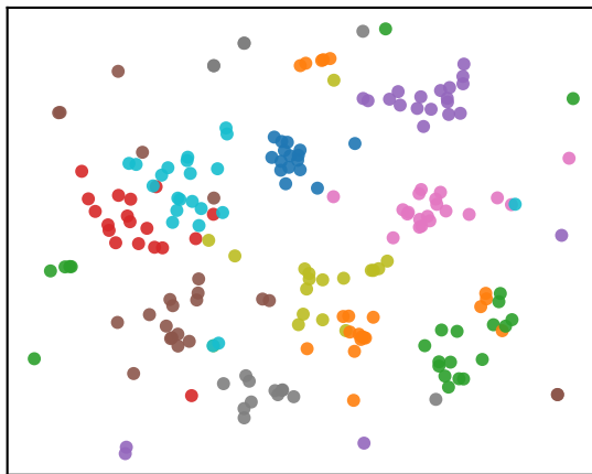
Fisher-Rao, noise=0.5
