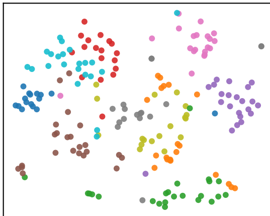
Fisher-Rao, noise=0.5
