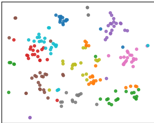
Fisher-Rao, noise=0.0
