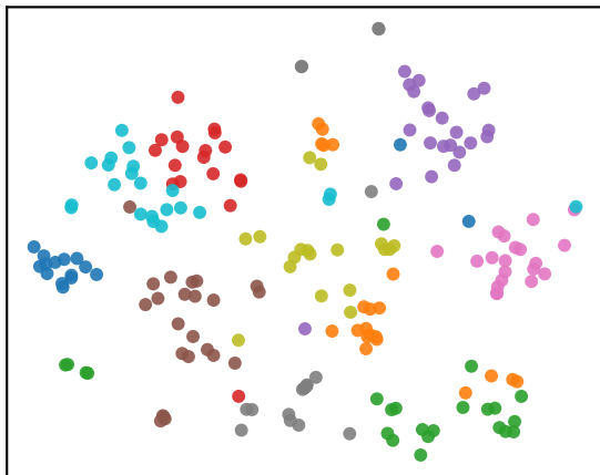
Fisher-Rao, noise=0.0
