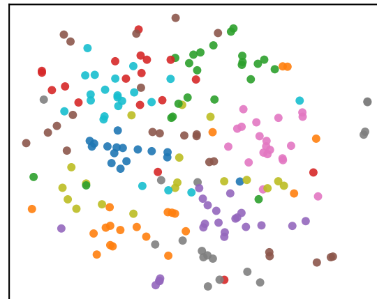
Fisher-Rao, noise=1.0
