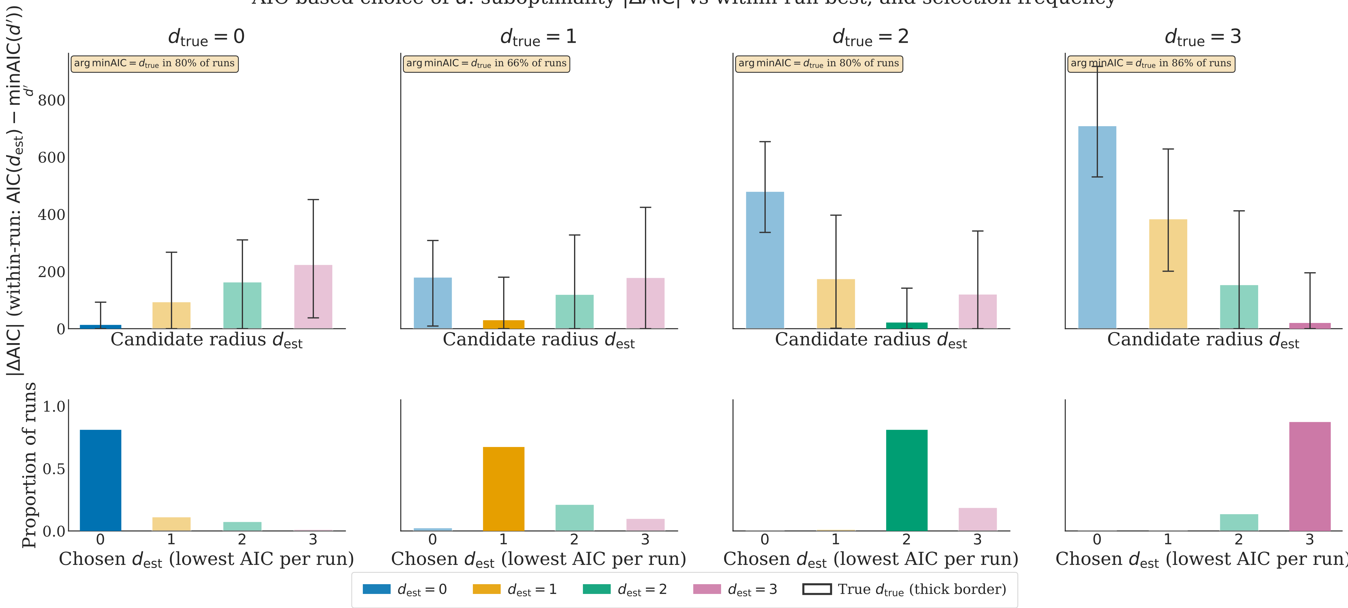
AIC-based choice of d : suboptimality |\Delta\text{AIC}| vs within-run best, and selection frequency
