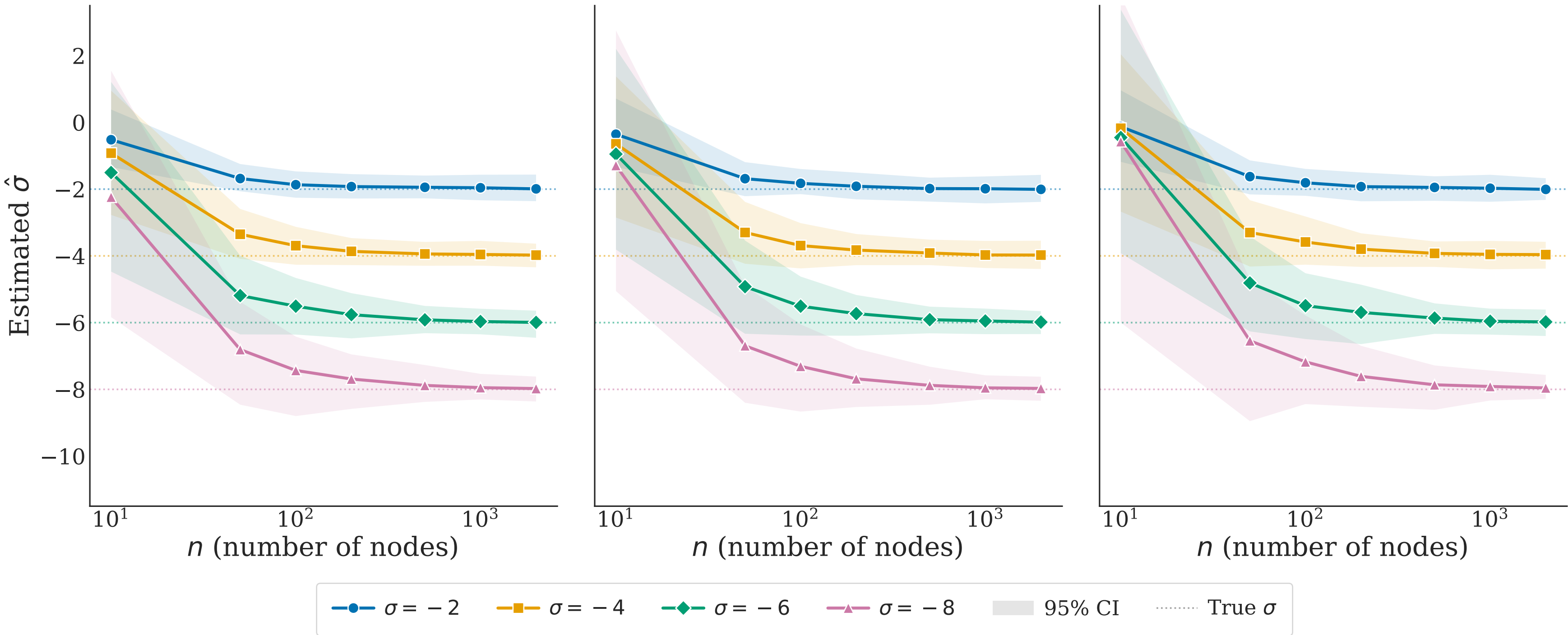
Convergence of \hat{\sigma} to the true parameter as n increases
