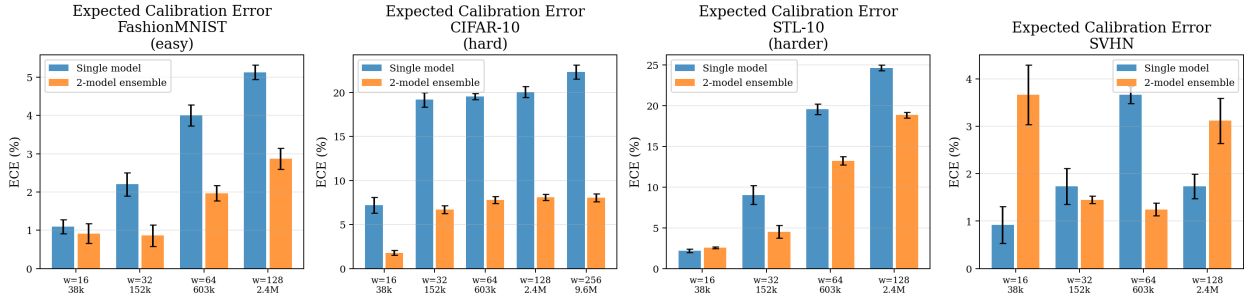
Figure 2: Expected Calibration Error (ECE) for individual models (blue) and two-member ensembles (orange) at each width. The calibration benefit of ensembles is 5–10 \times larger on CIFAR-10 than on FashionMNIST.
