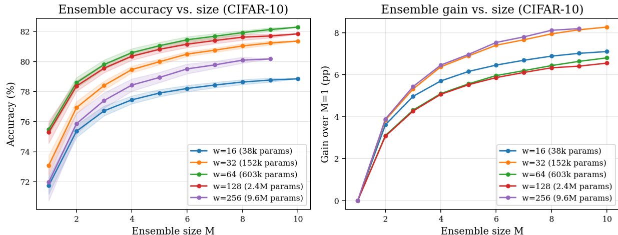
Figure 3: Ensemble accuracy (left) and gain over single model (right) as a function of ensemble size M on CIFAR-10, for each width. Shaded bands show \pm 1 std across bootstrap samples. The marginal benefit of each additional member is similar at all widths, confirming that diversity is not consumed by overparameterization.
