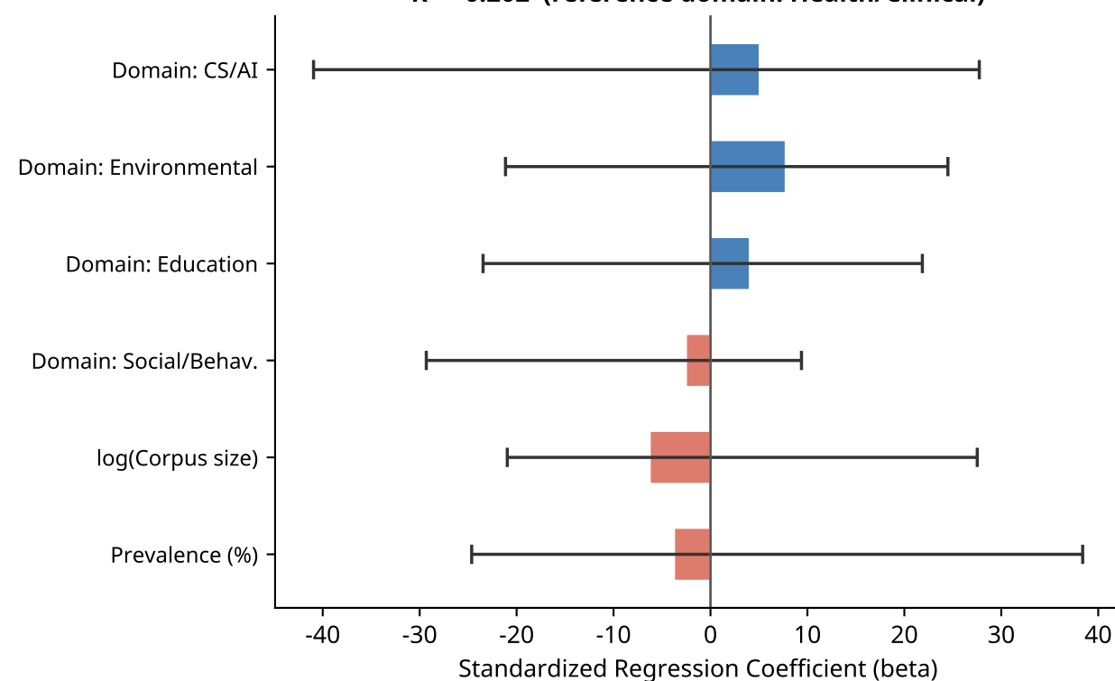
(d) Regression: WSS@95 ~ Prevalence + log(Size) + Domain R 2 = 0.202 (reference domain: Health/Clinical)
