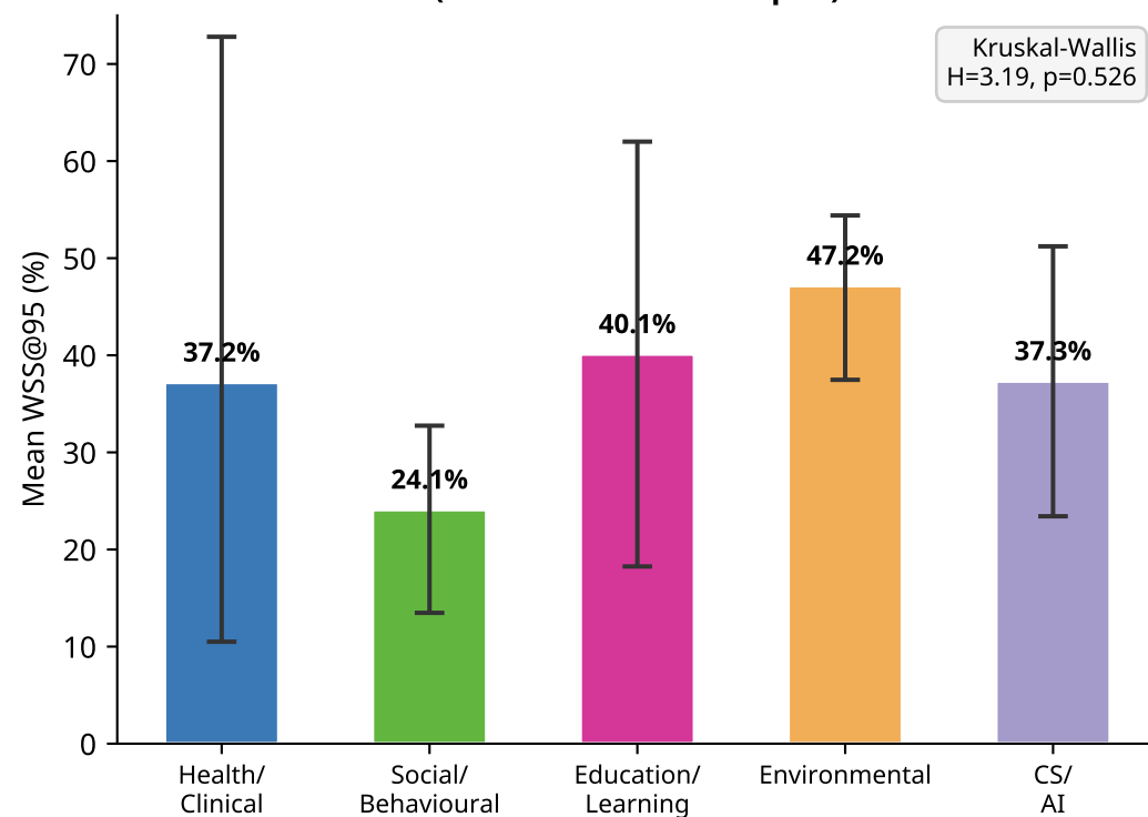
(a) Domain-Level WSS@95 (mean \pm 95% bootstrap CI)
