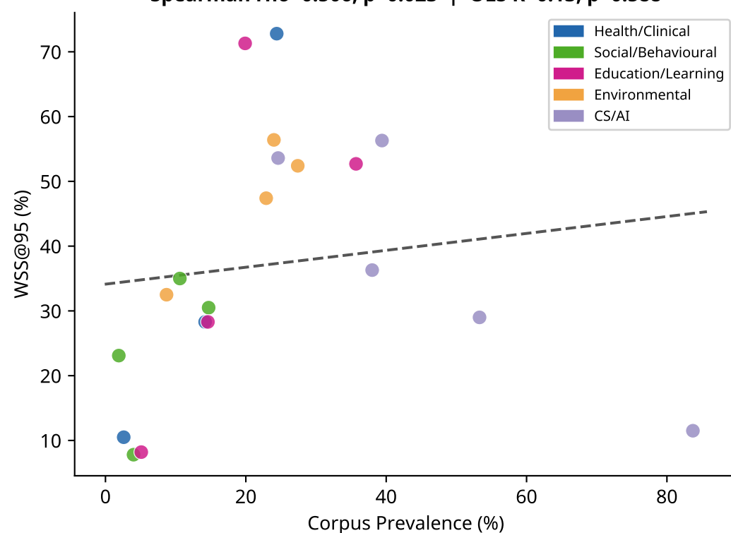
(c) Prevalence vs. WSS@95 Spearman rho=0.506, p=0.023 | OLS R=0.13, p=0.588
