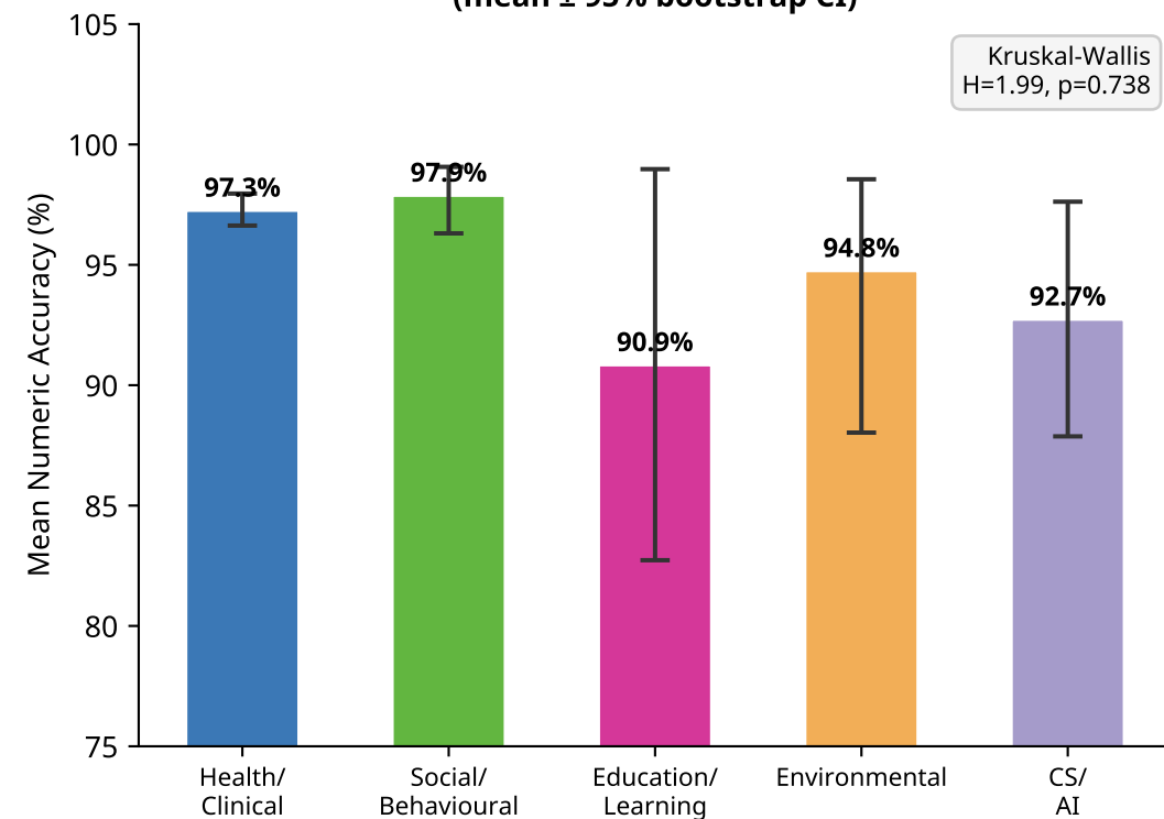
(b) Domain-Level Numeric Accuracy (mean \pm 95% bootstrap CI)
