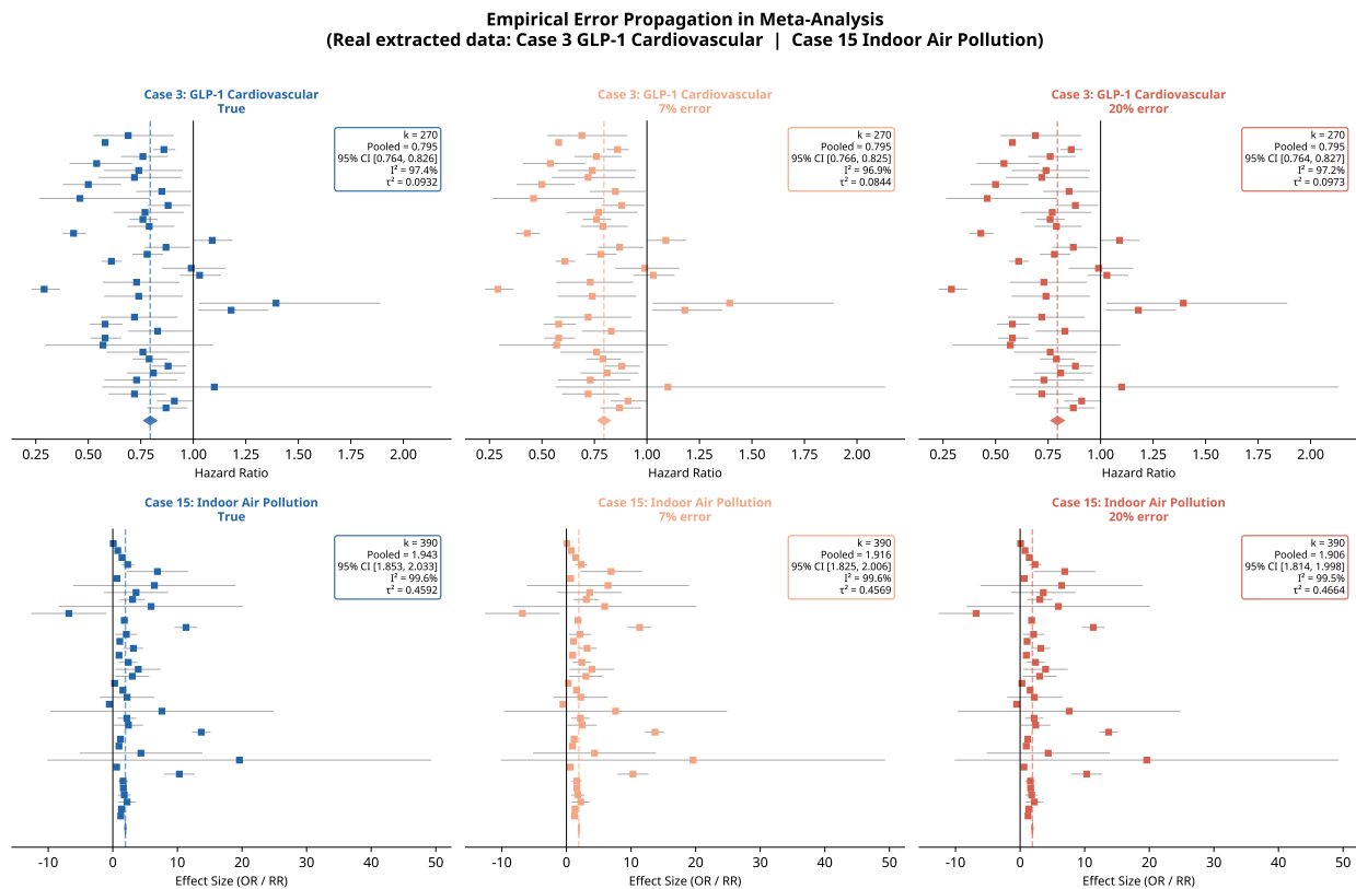
Figure 8: Empirical error propagation in meta-analysis computed from real extracted data across two case studies (Case 3: GLP-1 Cardiovascular Outcomes, k = 270 ; Case 15: Indoor Air Pollution, k = 390 ). The forest plots compare the true pooled estimate (computed from verified values) against 7% and 20% numeric error rates. Massive baseline heterogeneity ( I^2 > 95\% ) masks the extraction errors, resulting in stable pooled estimates despite variance inflation at the study level.
