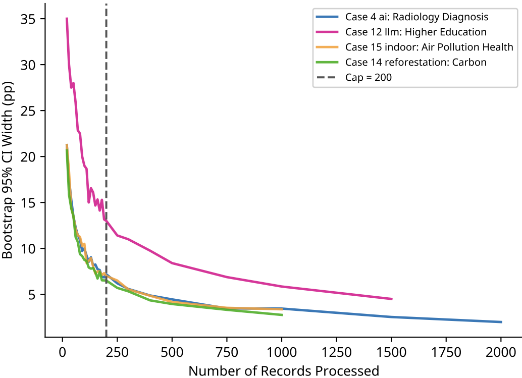
(c) CI Width Saturation (precision stabilises before 200 records)
