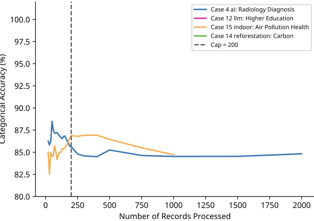
(a) Categorical Accuracy vs. Records Processed
