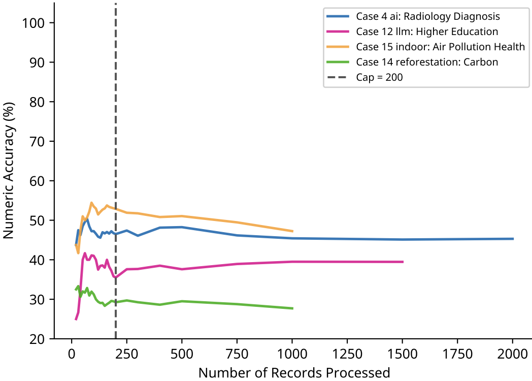
(b) Numeric Accuracy vs. Records Processed
