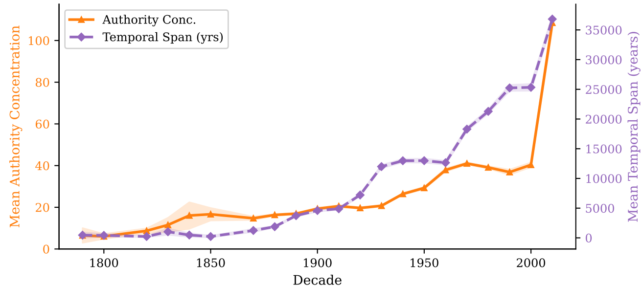
Authority Concentration and Temporal Span over SCOTUS History
