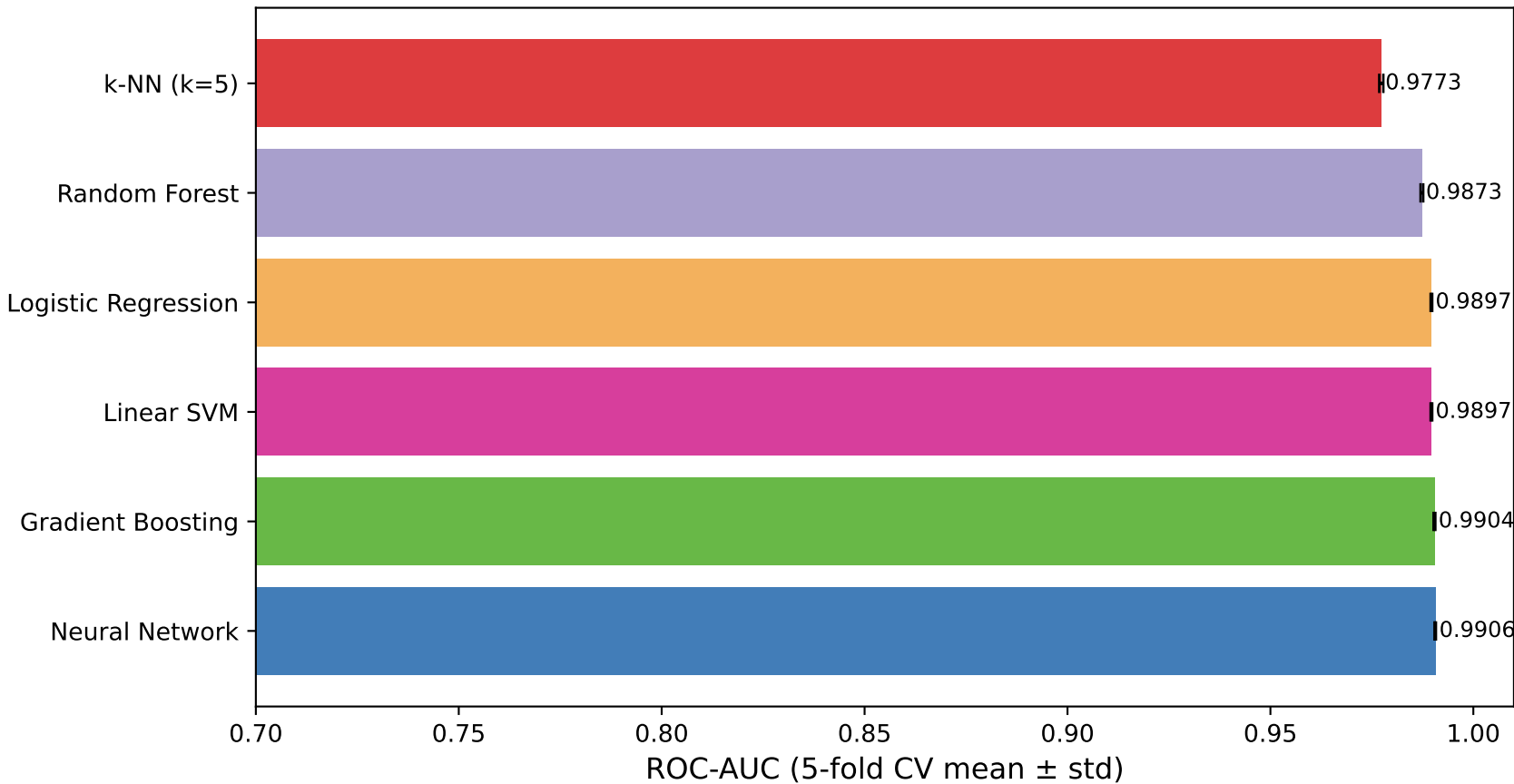
Model Comparison: Citation Prediction Performance (LIS)
