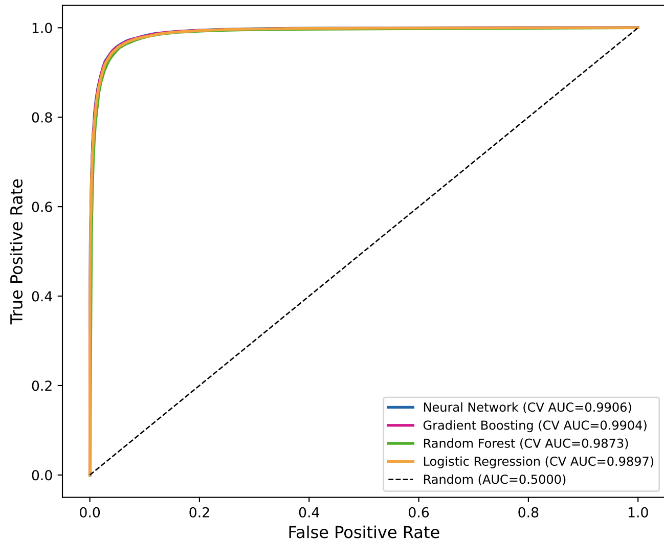
ROC Curves — LIS Citation Prediction
