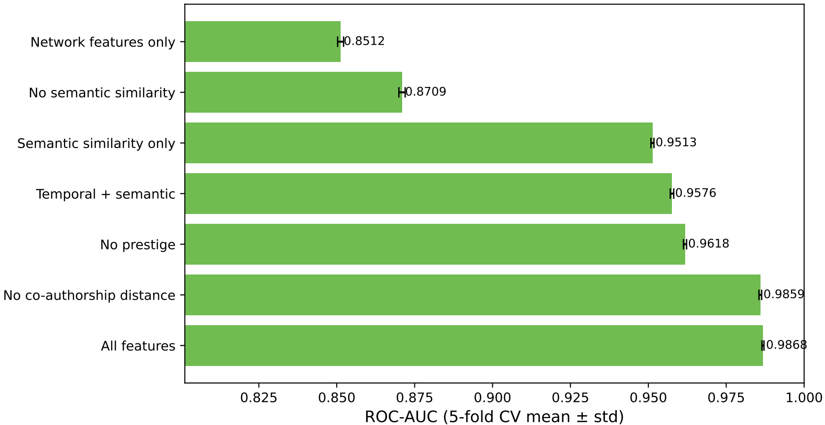
Ablation Study: Feature Subset Importance (Random Forest) — LIS
