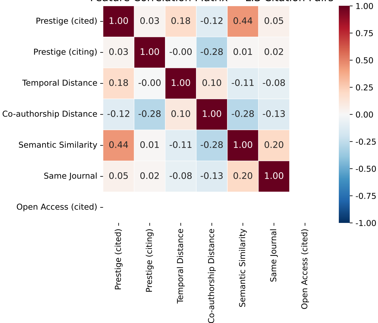
Feature Correlation Matrix — LIS Citation Pairs
