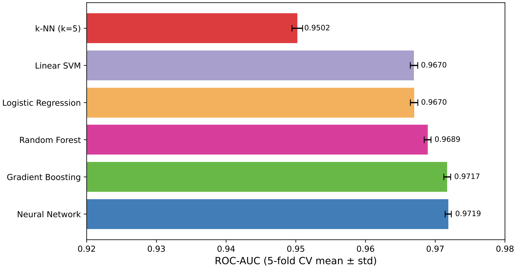
Model Comparison: ROC-AUC
