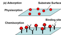
Figure: Types of adsorption [5].
