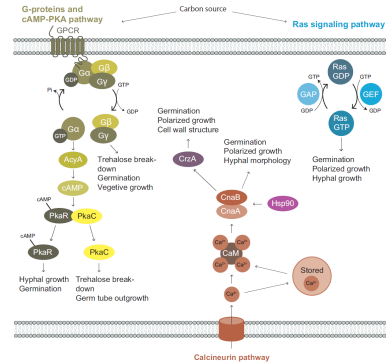
Figure: Carbon signalling pathways [1]
