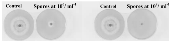
Figure: Auto-inhibition through spore density [2]
