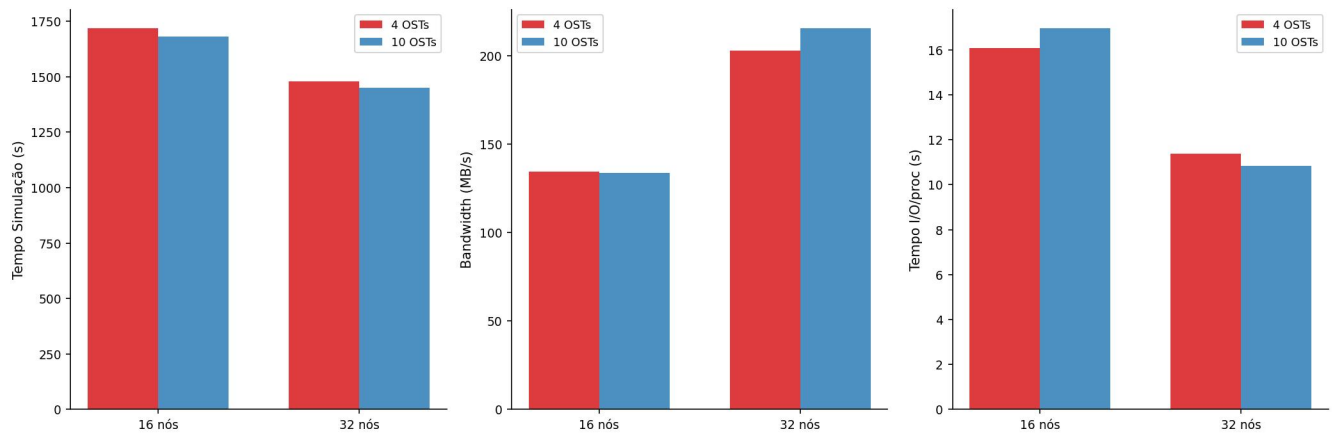
AWS MPI-IO: 4 OSTs vs 10 OSTs (16 e 32 nós)
