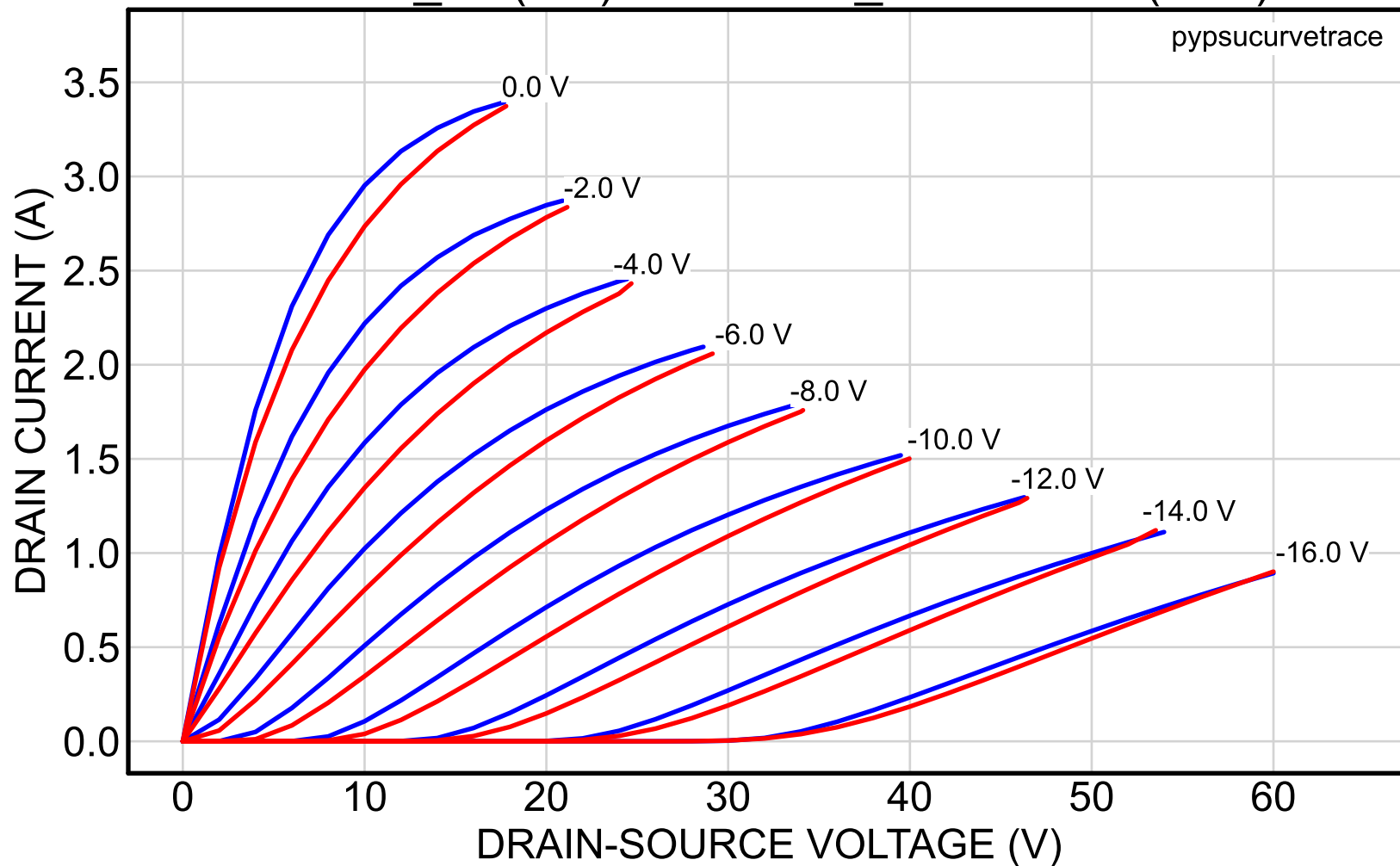
2SK82_10 (red) vs. 2SK82_39reserved (blue)
