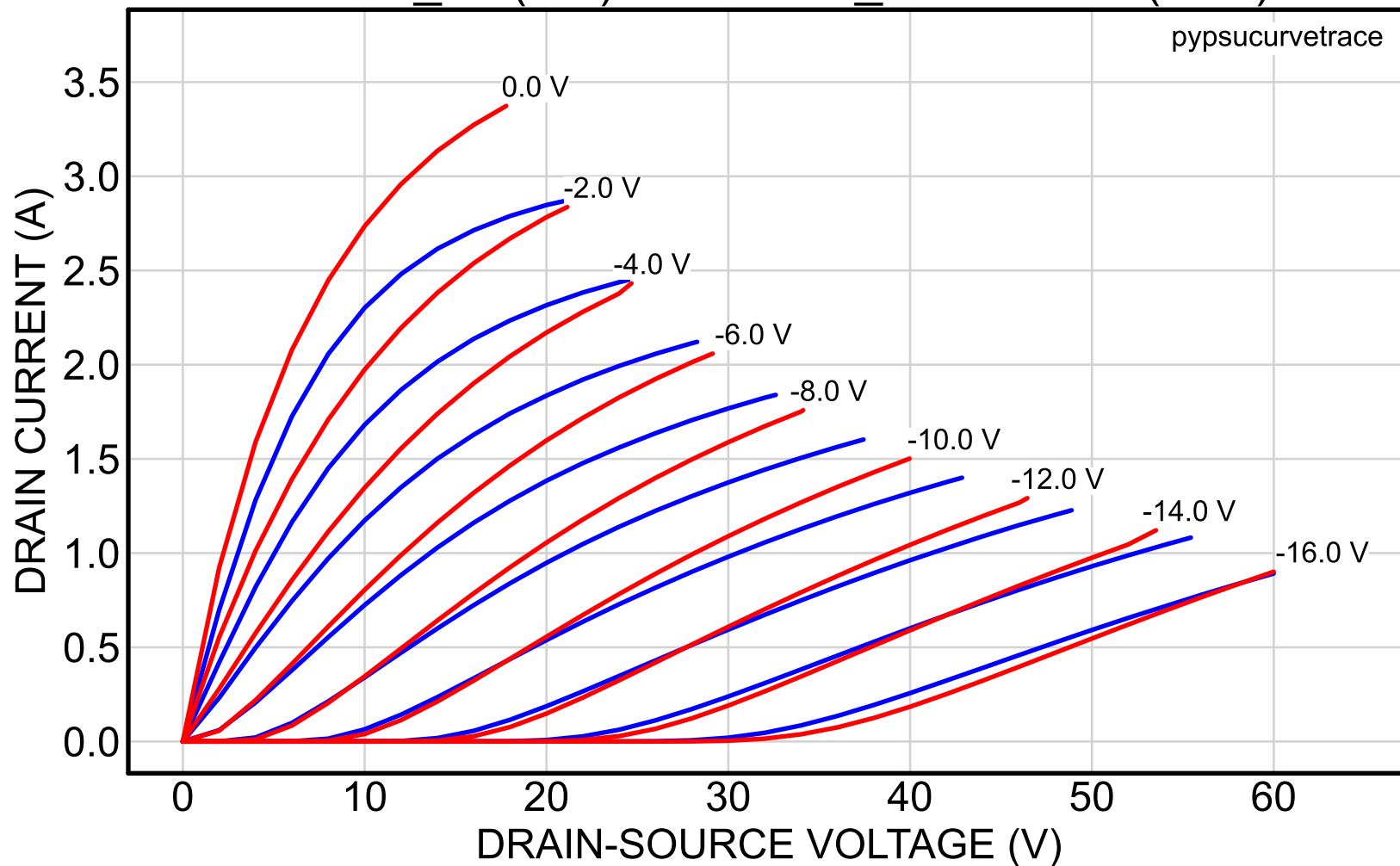
2SK82_10 (red) vs. 2SK82_40reserved (blue)
