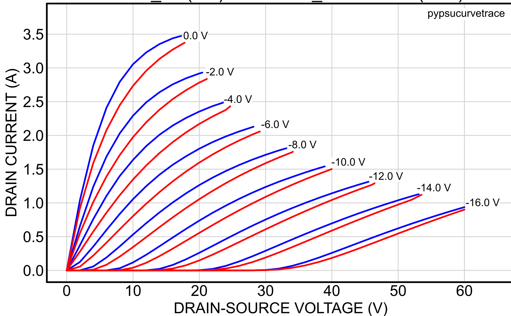
2SK82_10 (red) vs. 2SK82_52reserved (blue)
