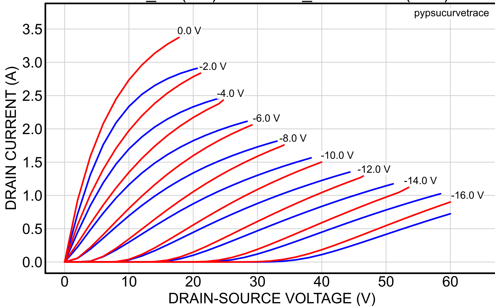
2SK82_10 (red) vs. 2SK82_56reserved (blue)
